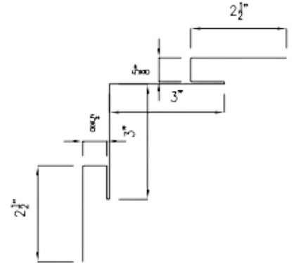
Inside Corner
