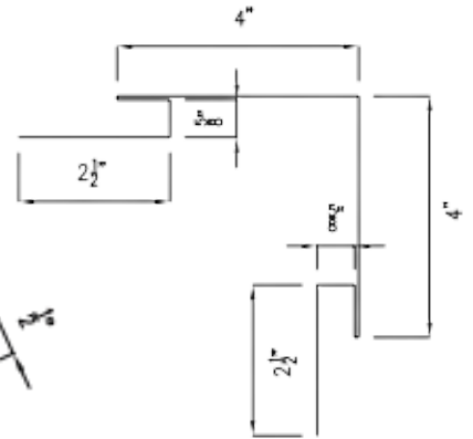
Double J-Trim
