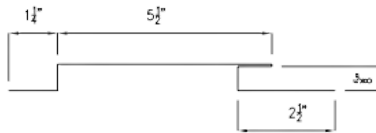
5 1/2 Bond Board
