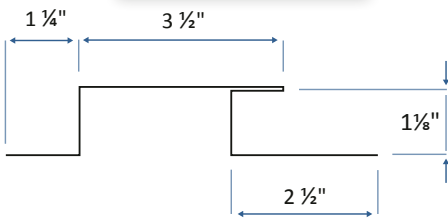
Accent 3 1/2 Band Board
