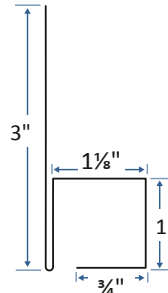
Accent Horizontal Base Trim
