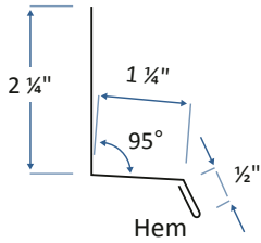
Accent Drip Cap - 1 1/4"
