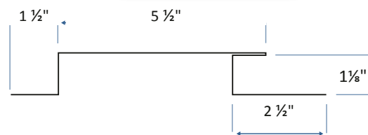
Accent 5 1/2 Band Board
