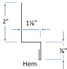
Accent Double Angle Trim
