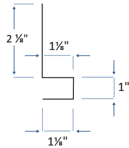
Accent Double Angle Trim
