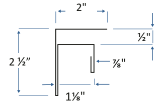
Accent Double J-Trim
