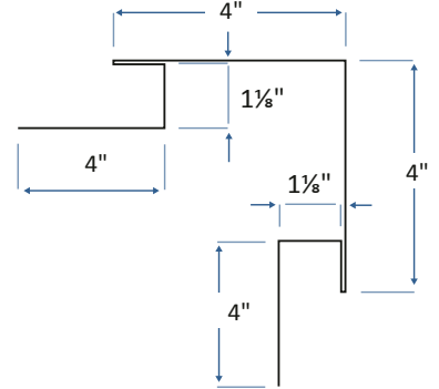
Accent Double J-Trim
