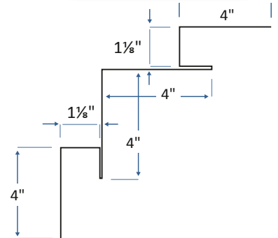
Accent Inside Corner
